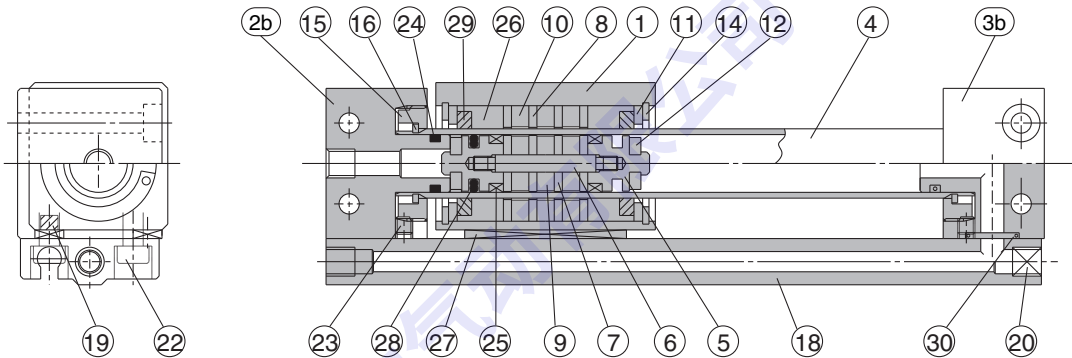
CY3RG15~63
